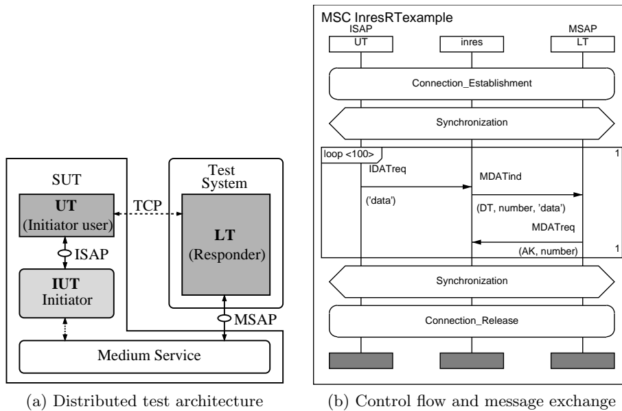
Figure 1: Test architecture and control flow for the Inres test case example
